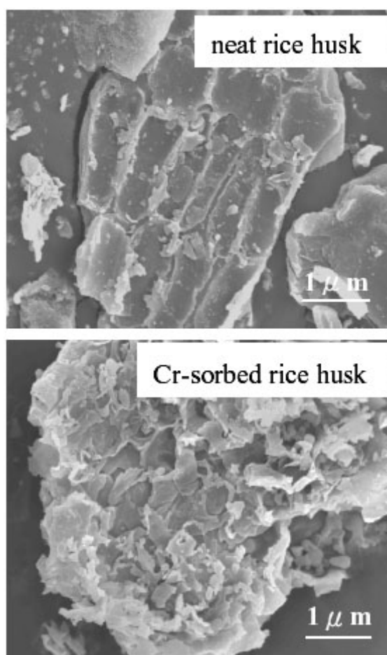
Figure 1. SEM morphologies of the neat rice husk (top panel) and the rice husk having sorbed Cr(VI) in the 2000 mg Cr l -1 solution for 48 h (bottom panel).
