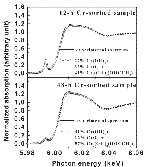
Figure 3. Results of the simulation of sample XANES spectra (top: the 12 h sample; bottom: the 48 h one) with that of three references: \text{CrO}_3 , \text{Cr(OH)}_3 and \text{Cr}_3(\text{OH})_2(\text{OOCCH}_3)_7 .
