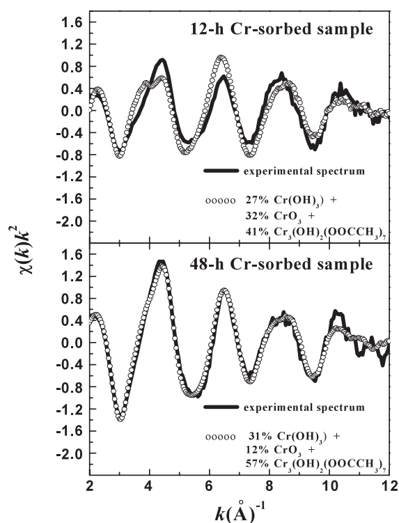
Figure 4. Simulation of the sample EXAFS spectra of Cr-sorbed rice husks with that of three references: \text{CrO}_3 , \text{Cr}(\text{OH})_3 and \text{Cr}_3(\text{OH})_2(\text{OOCCH}_3)_7 .
